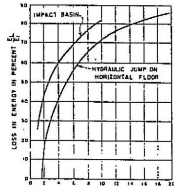
COMPARISON OF ENERGY LOSSES
