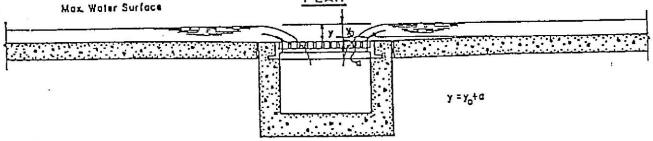
DROP INLET (Grate covering) Type A-5
