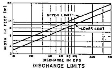
DISCHARGE LIMITS
